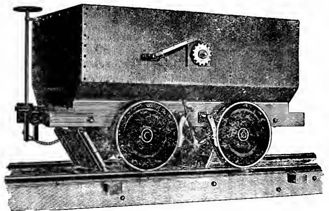
Fig. 31. CEMENT CAR, DROP BOTTOM, BUILT BY BLOOMSBURG CAR COMPANY.
